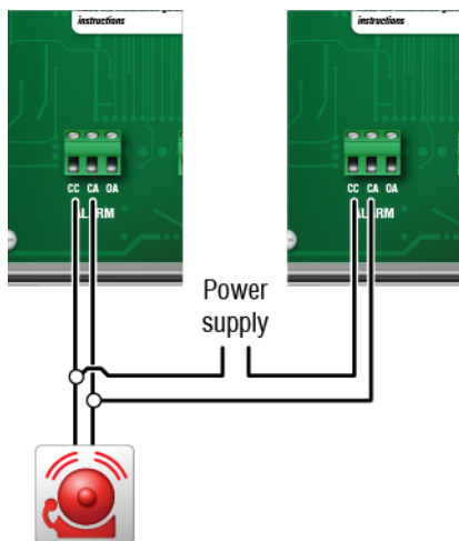
Normally open system (closed on alarm)
