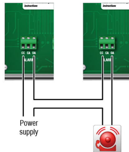
Normally closed system (open on alarm)
